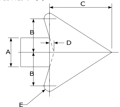
D.O.T. D-15 ARROWHEAD DETAIL N.T.S.
