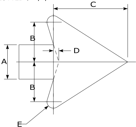
D.O.T. D-15 ARROWHEAD DETAIL N.T.S.
