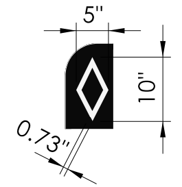
SIGN NUMBER 31-0905 PANEL SIZE 5'-0" x 3'-0" SIGN AREA 15.0 Sq.Ft. MUTCD R3-10 (CT) BDR INSET/WIDTH 1" / 1" CORNER RADIUS 5" BACKGROUND TYPE: * COLOR: White LEGEND/BORDER TYPE: * COLOR: Black / Black * REFER TO CATALOG OF SIGNS FOR SHEETING TYPE. WHEN COLOR IS BLACK TYPE IS "PLAIN".
