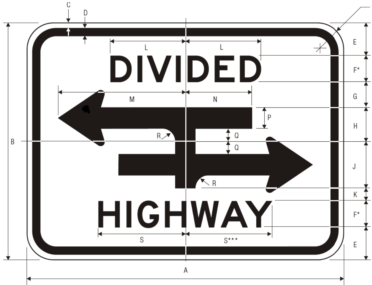
R6-3a DIVIDED HIGHWAY CROSSING
