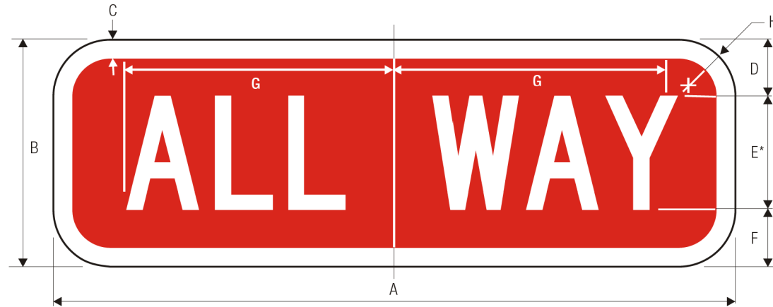
R1-4 ALL WAY
