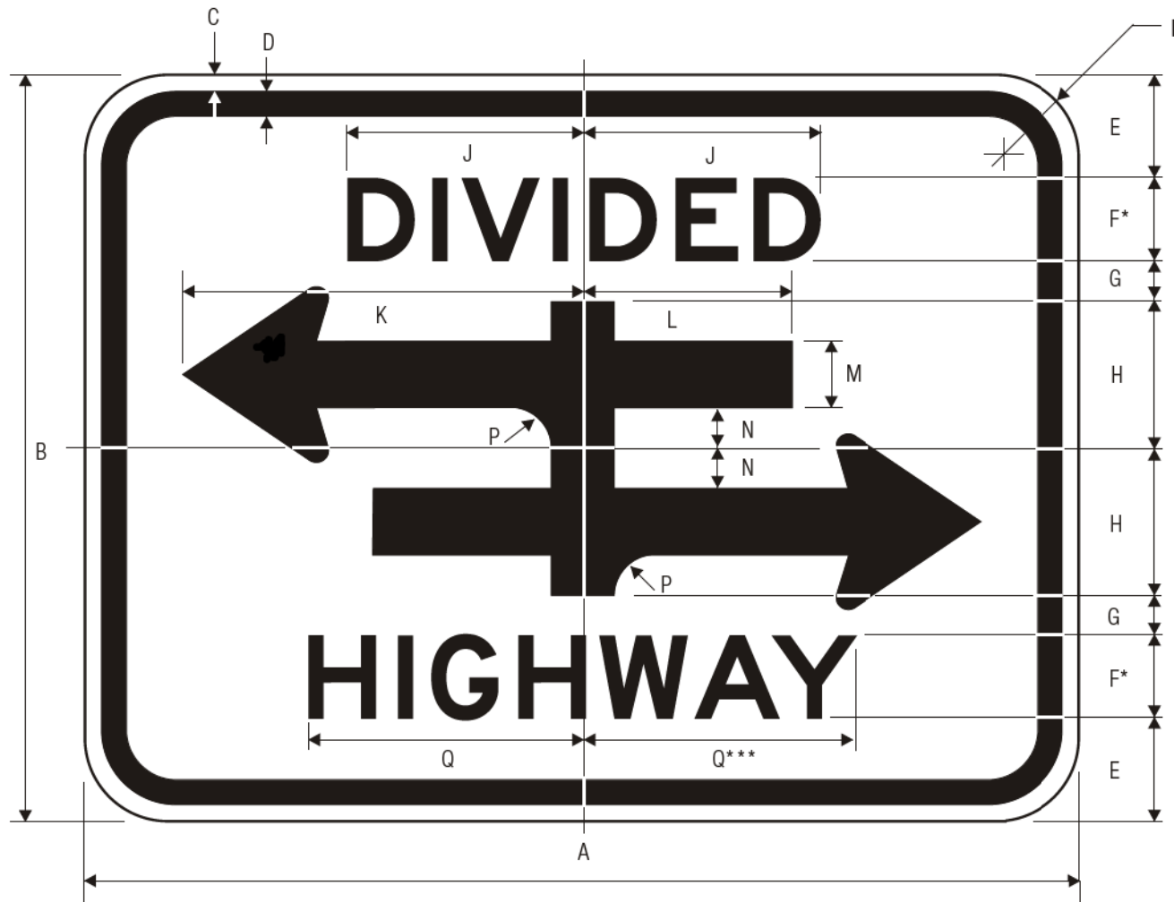
R6-3 DIVIDED HIGHWAY CROSSING
