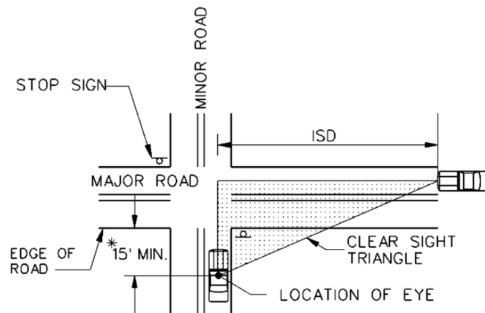
CLEAR SIGHT TRIANGLE FOR VIEWING TRAFFIC APPROACHING FROM THE RIGHT
