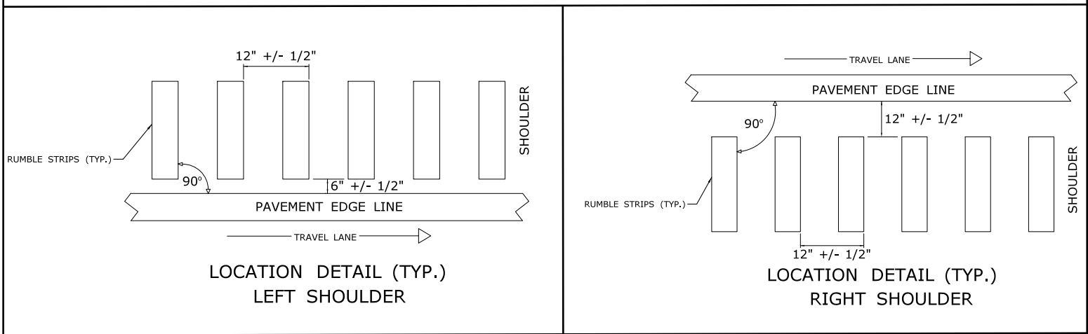
Figure 4.07-1: DETAILS AND SECTIONS OF RUMBLE STRIPS
