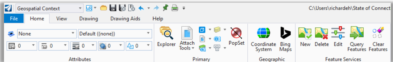
Figure 130 – Geospatial Workflow
