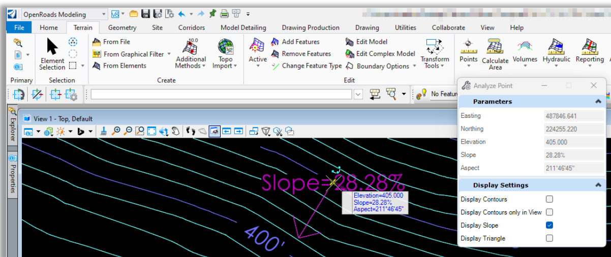
Figure 128 – Analyze Point
