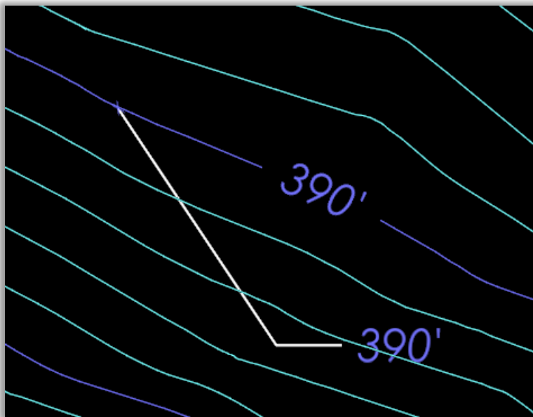
Figure 127- Label Terrain Spots
