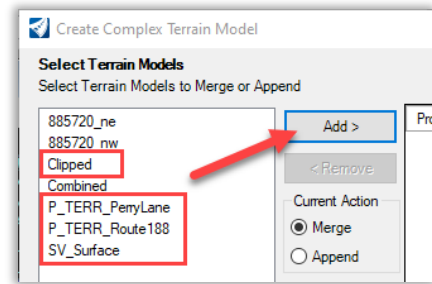
Figure 120 – Add Terrains
