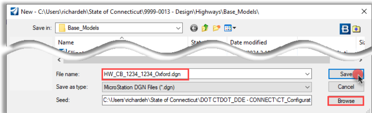
Figure 44 – New File
